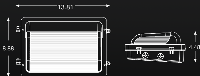
CWPS-40W-3P-3CCT-UD CWPS-80W-3P-3CCT-UD
